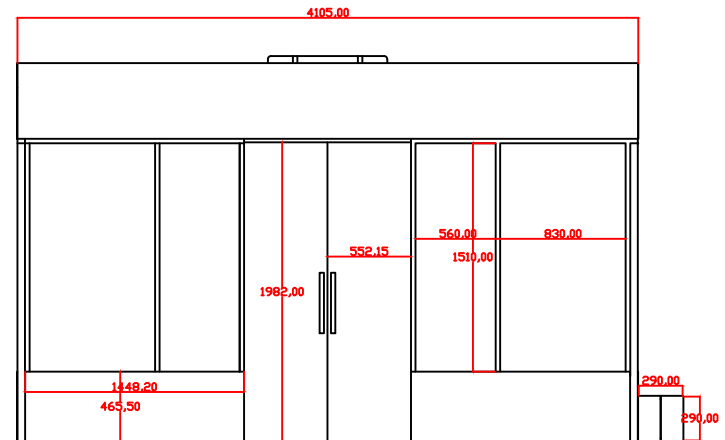
VISTA FRONTAL
